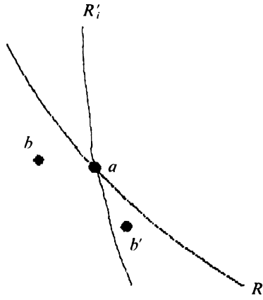
FIGURE 2 Single-crossing preferences
